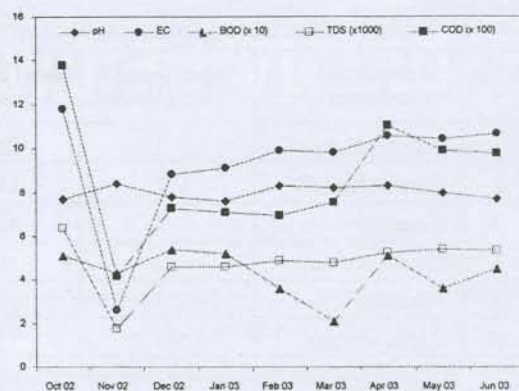
Figure 5: Monthly variation in pH, EC (mS/cm), BOD (mg/L), TDS (mg/L) and COD (mg/L) of leachate collected from borehole 6 of Perungudi.
